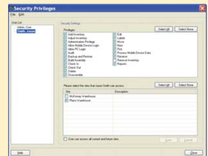
▶ Feature-based security
